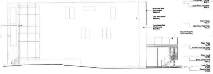
3 East Elevation 1/8" = 1'-0"
