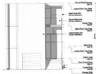
1 South Elevation 1/8" = 1'-0"
