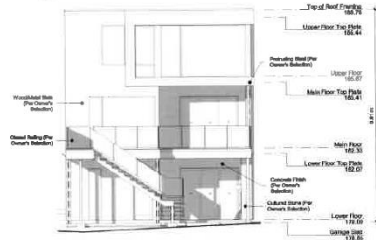
2 North Elevation 1/8" = 1'-0"
